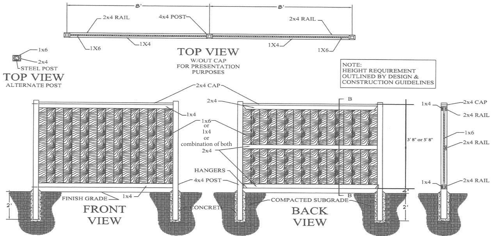
GOOD NEIGHBOR/PERIMETER DOUBLE RAIL
